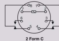
2 Form C
