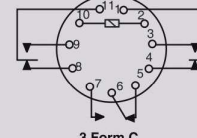
3 Form C
